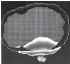
Radiation penetration in head of adult
