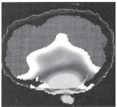
Radiation penetration in head of 10 year old child
